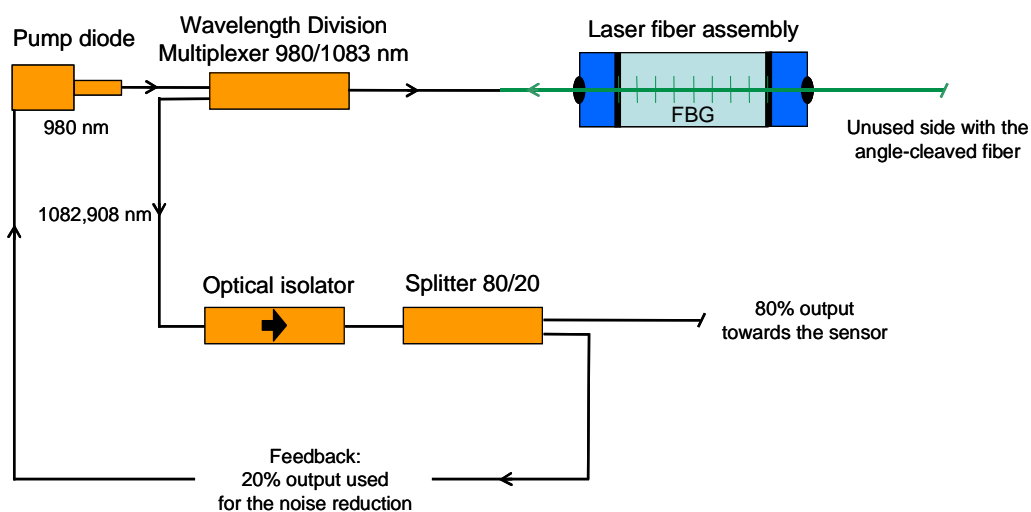
Fig. 1. Laser architecture
