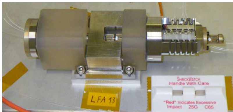
Fig. 2. Photography of a LFA: the pre-stressed piezoelectric actuator on the right is glued on the Zerodur ® ; the LFA is then fixed in the ASM electronics box with the titanium bridge put upon the Zerodur ®
